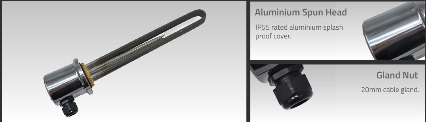
TYC Range - K Lid with TSDR Thermostat
