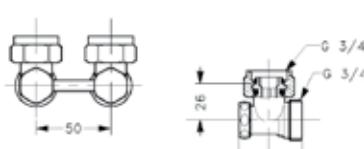
RLV-KS back connection, 3/4" internal connection
