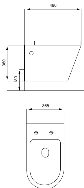
Rimless Wall Hung WC Pan
