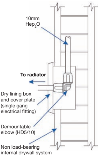
Fig. 56 Radiator connection using 10mm Hep 2 O and a dry lining box within a drywall
