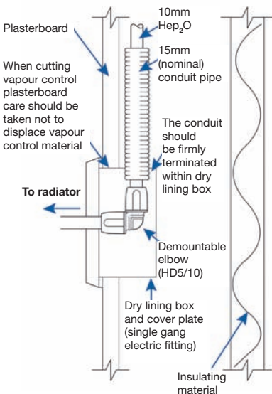
Fig. 57 Radiator connection using 10mm Hep 2 O within timber or steel framed external wall
