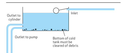
Figure 1: Tank inlet and outlet position
