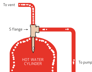
Figure 25: S flange
