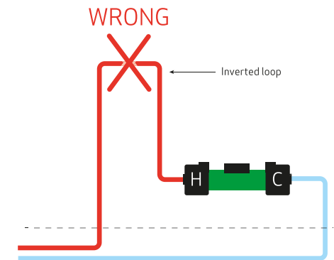
Figure 27: Inverted loops
