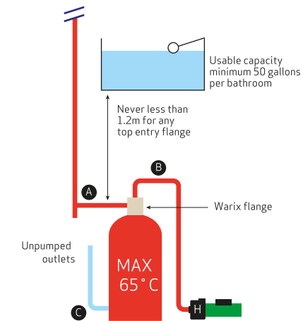
Figure 26: Approved flanges
