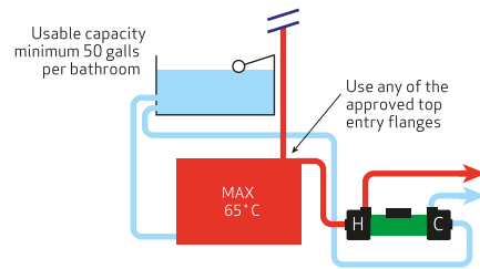
Figure 24: Horizontal cylinders
