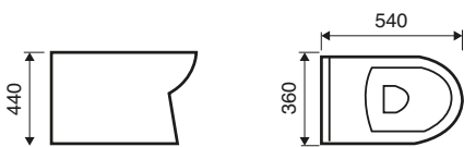
WWB-KBP0T730LS Comfort Height Back to Wall Pan
