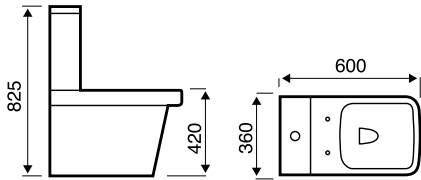
WWB-KBPOT400S1 Premier Close Coupled Pan
