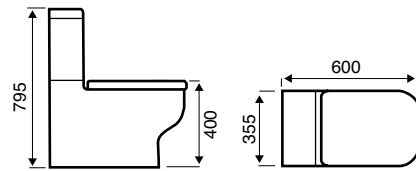
WWB-KBP0T0700P Close to Wall Close Coupled Pan
