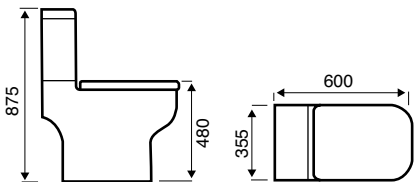
WWB-KBP0T0890P Comfort Height Close Coupled Pan
