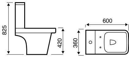
WWB-KBPOT405S1 Close Coupled Pan
