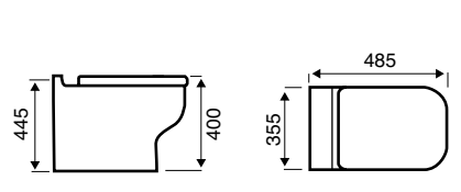
WWB-KBPOT0710P Back to Wall Pan
