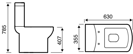
WWB-KBPOT601AS Close Coupled Pan
