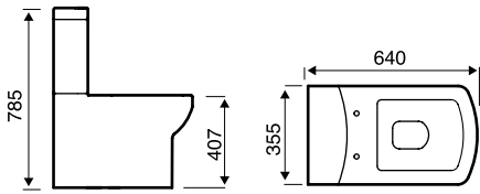
WWB-KBPOT602AS Close to Wall Close Coupled Pan
