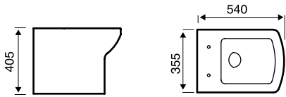
WWB-KBPOT604AS Back to Wall Pan
