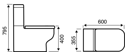
WWB-KBPOT0700P Close to Wall Close Coupled Pan
