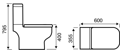
WWB-KBPOT0800P Close Coupled Pan
