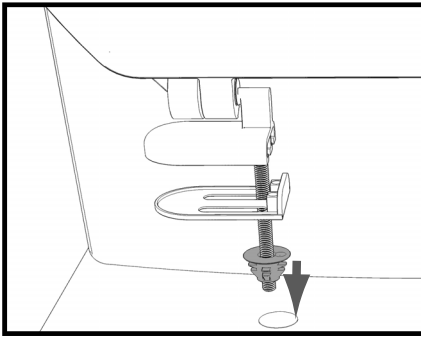
STEP 1 HINGE ASSEMBLY
