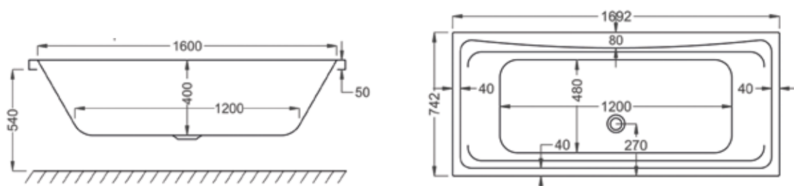
Tarn 1700 x 750mm Double End
