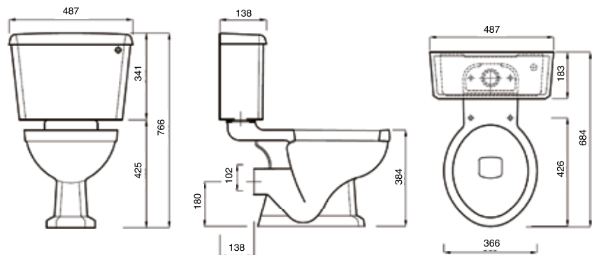
Close Coupled WC Pan & Cistern
