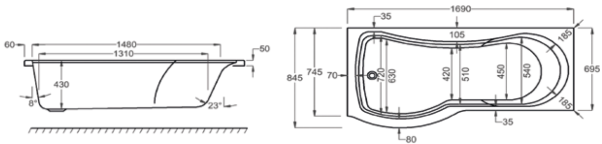
Fitou 1700 x 850mm
