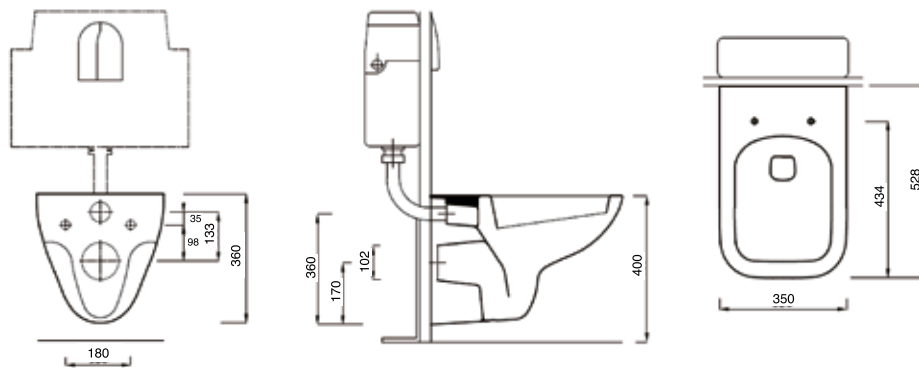
Square Wall Hung WC Pan
