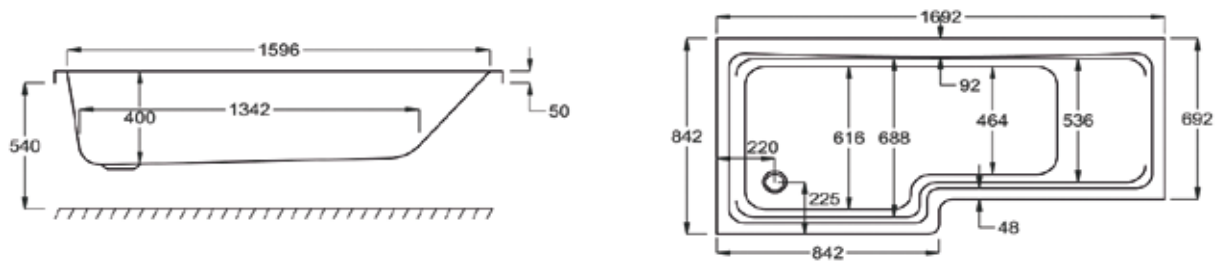
Fitou 1700 x 850mm
