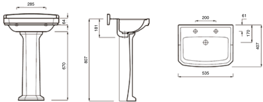
53cm Wash Basin & Pedestal
