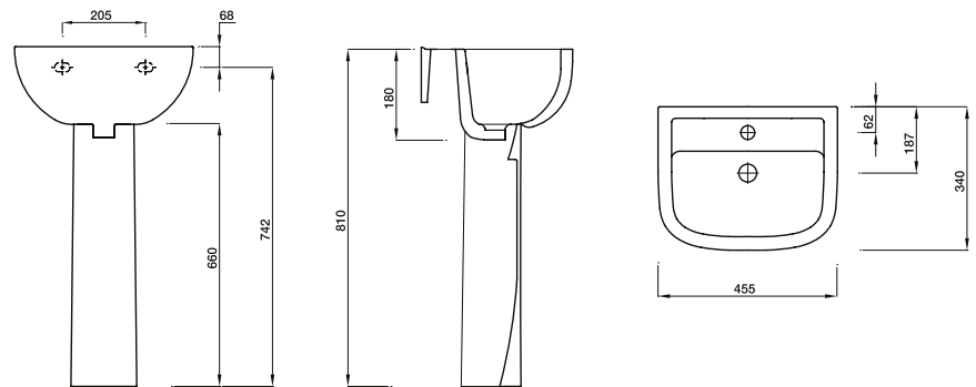
55cm Basin & Pedestal
