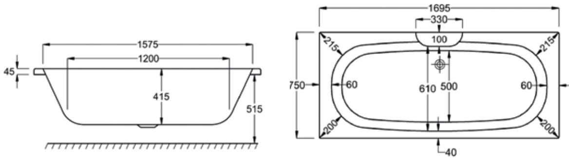
Laval 1700 x 850mm
