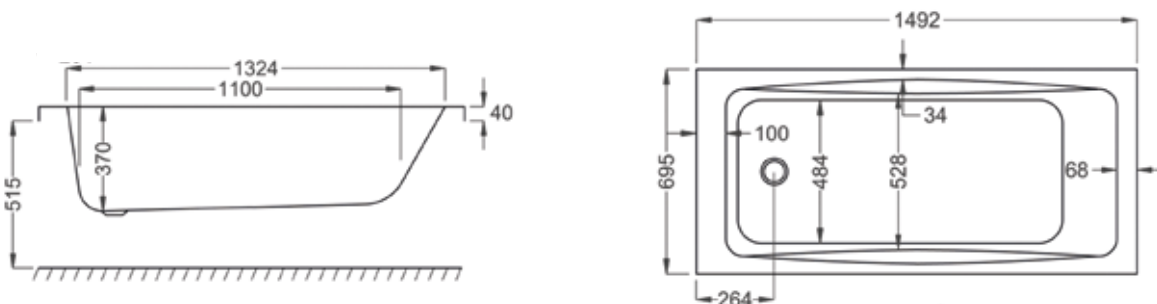
Burgos 1600 x 700mm
