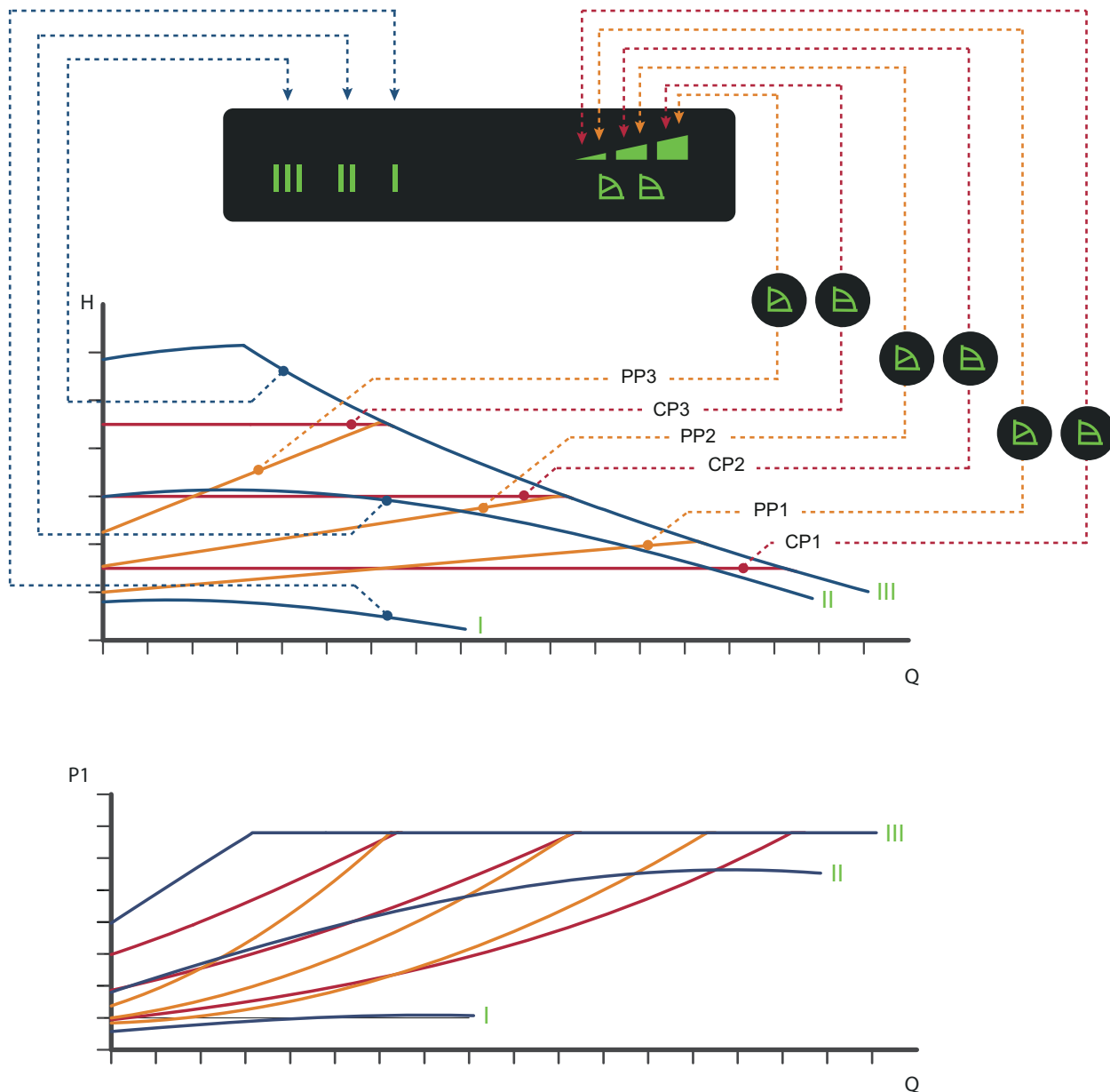
Fig. 21 Performance curves in relation to control modes
