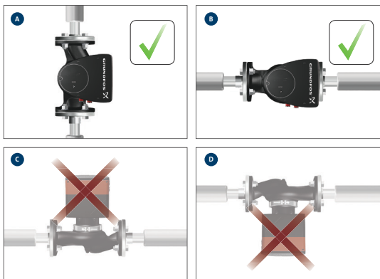
Fig. 9 Installation positions
