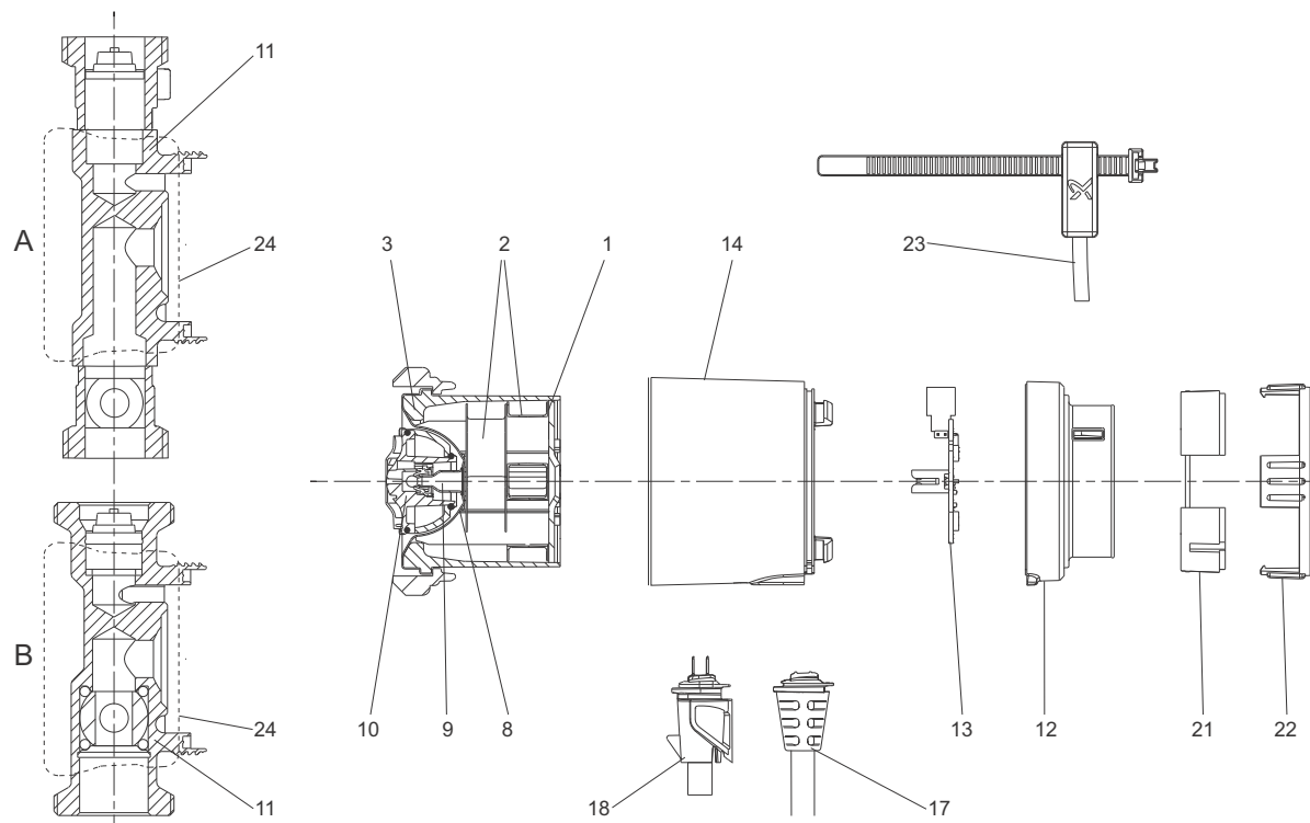
Fig. 19 Sectional drawing of COMFORT PM
