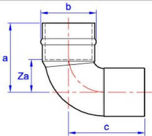
YP12S Elbow
