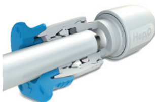
Figure 20: Cut-away drawing of HepKey™
