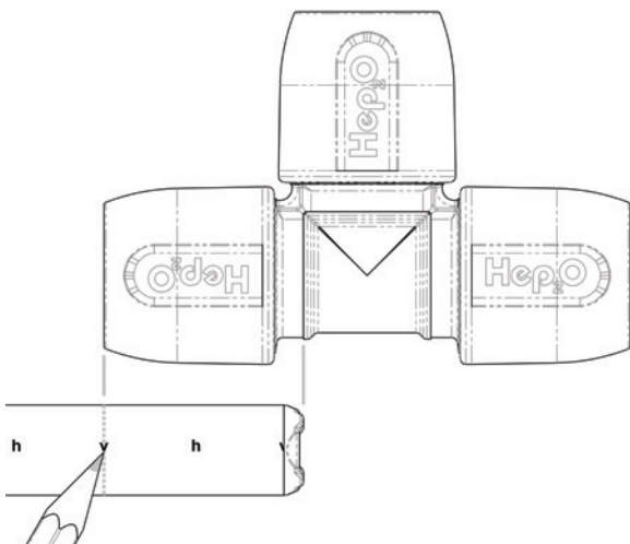
Figure 8: Hep 2 O 15mm assembly with pipe markings
