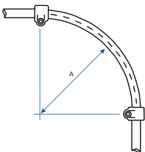
Figure 37: Minimum bending radii (8x pipe diameter)
