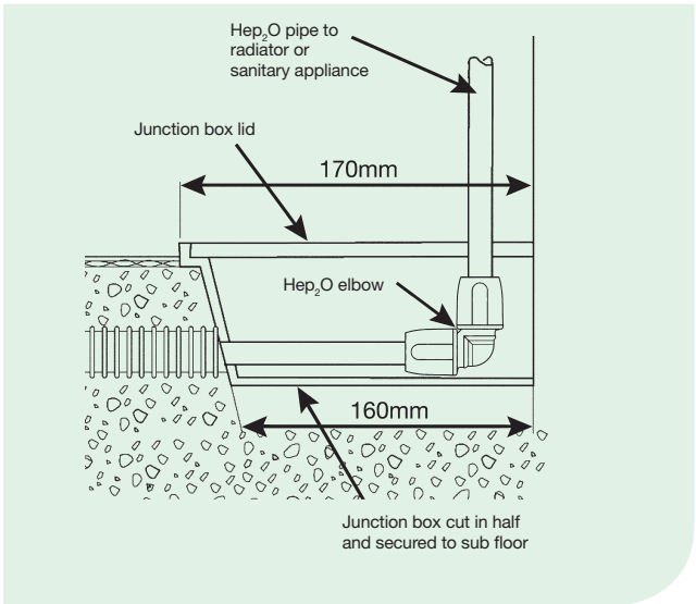
Figure 42: Cut junction box
