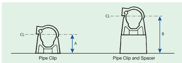
Figure 35: Pipe fixing centres
