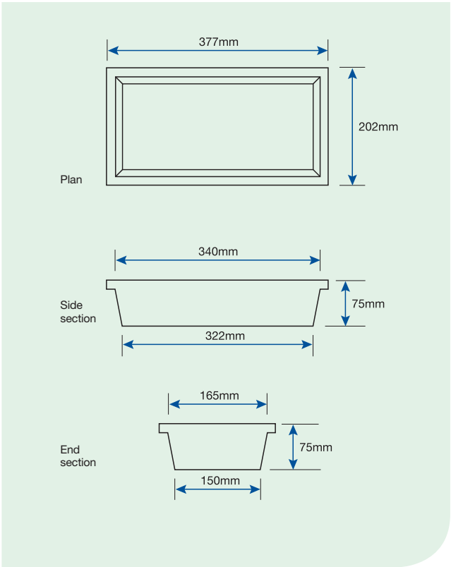
Figure 41: Junction box dimensions
