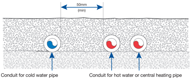
Figure 44: Spacing for cold water conduit in floor screeds
