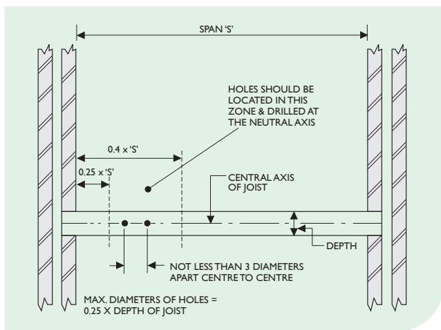
Figure 32: Explanation of drilling joists in accordance with the Building Regulations Approved Document A
