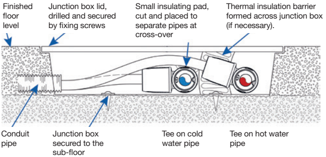
Figure 43: Hot and cold water distribution pipes at tees
