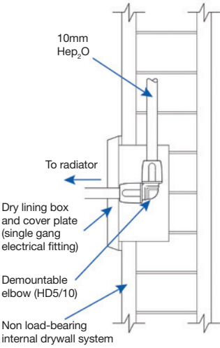
Figure 56: Radiator connection using 10mm Hep 2 O and a dry lining box within a drywall
