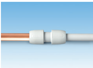
Figure 12: Hep 2 O fittings are also compatible with copper pipe
