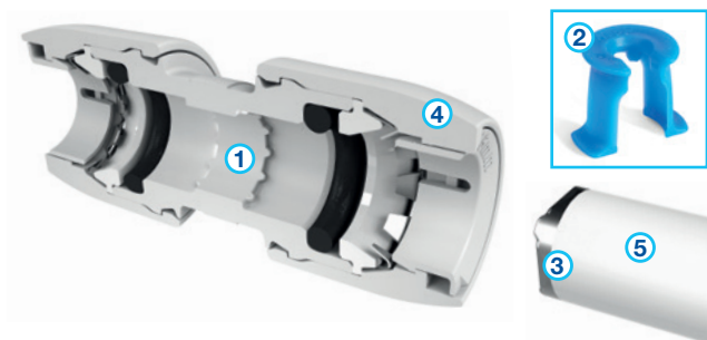
Figure 2: Cross section of Hep 2 O fitting
