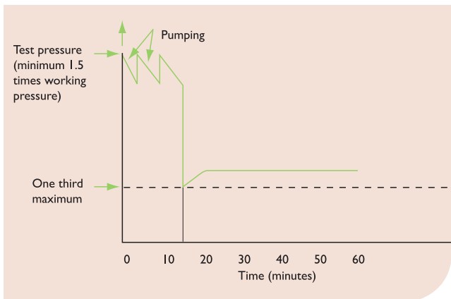
Figure 60: Test procedure
