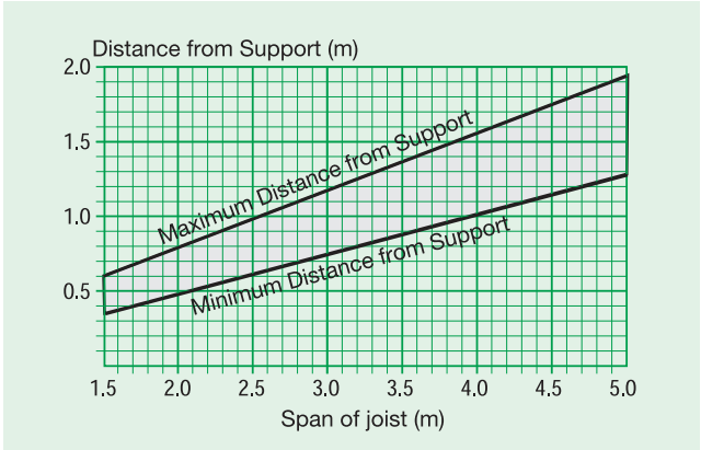
Figure 33: Graph showing dimension of joist drilling zone from support
