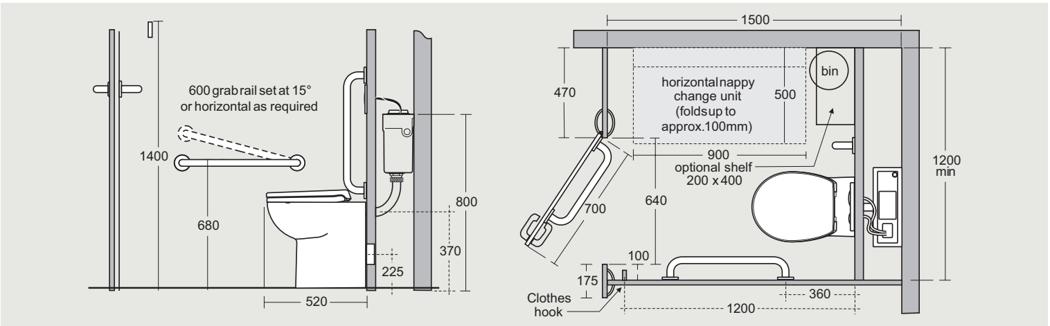
Ambulant disabled cubicle solution
