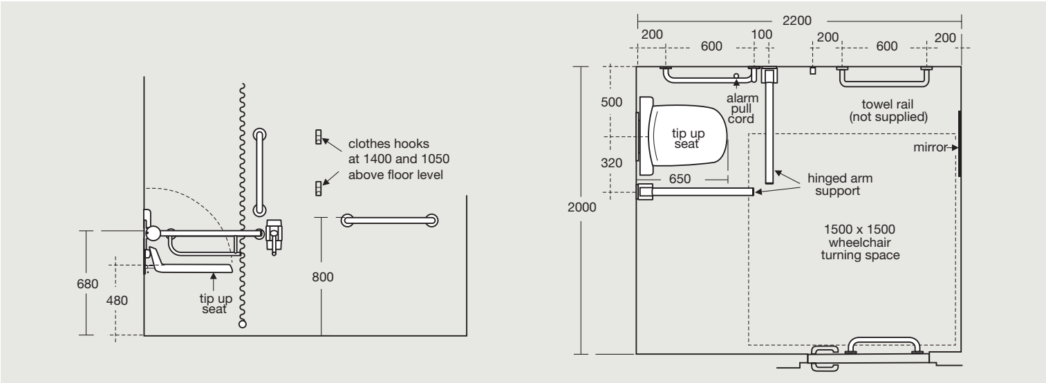
Public shower facilities solution
