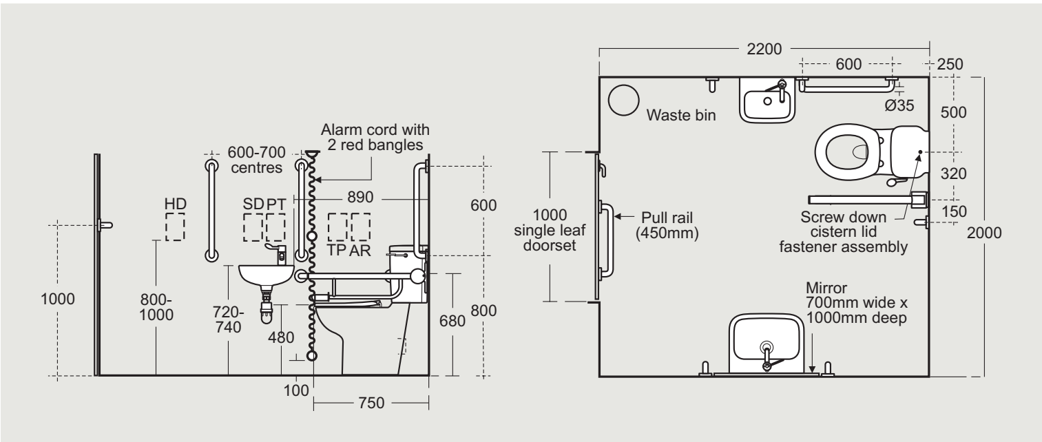
Large Unisex washroom for single toilet solution
