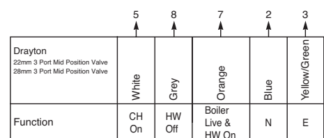
Motorised Valve
