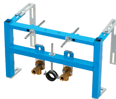
Passes 400Kg load test.
