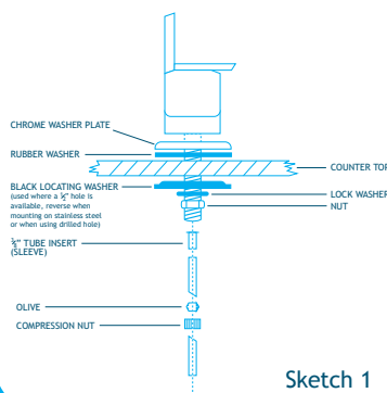
ASSEMBLE HARDWARE AS SHOWN
