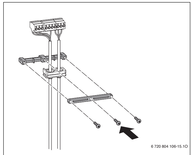
Fig. 17 Electrical connection - step 7
