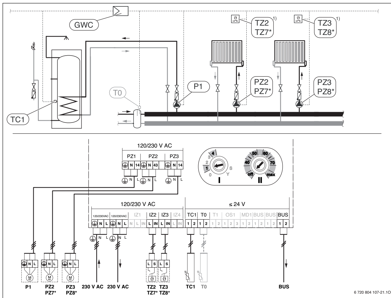
Fig. 23 Two heating circuits and one domestic hot water cylinder circuit
