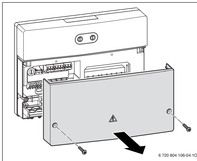
Fig. 4 Wall mounting - step 1
