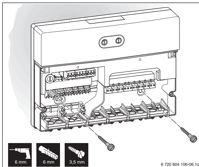
Fig. 6 Wall mounting - step 3
