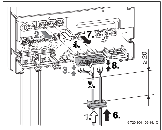
Fig. 16 Electrical connection - step 6
