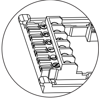
Dual Channel: MiTime T720R, T720M
