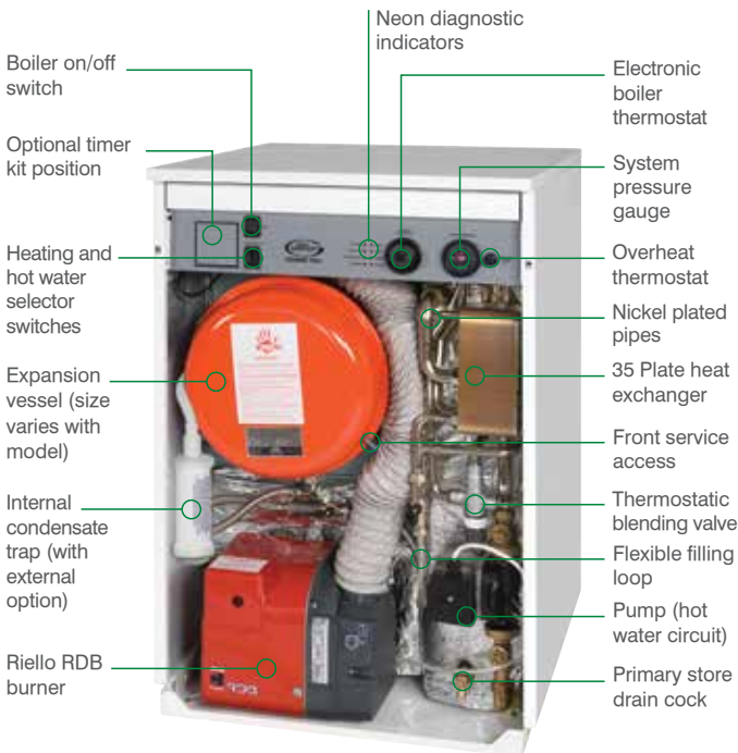
Model shown: VTXCOMBI26 (front view)
