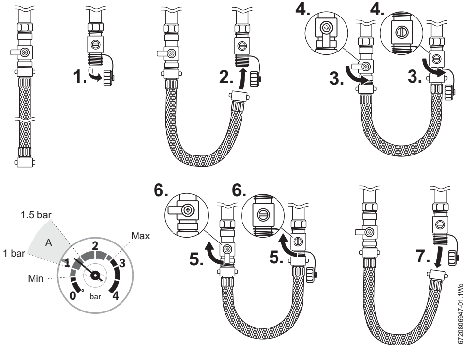
Fig. 5 External filling loop
