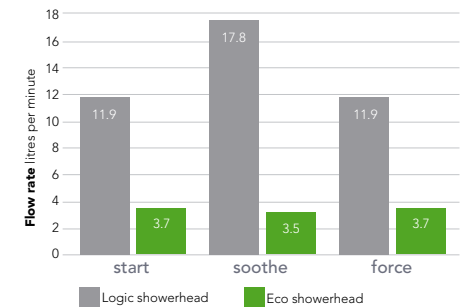
Flow rates at 0.5 bar Logic showerhead vs. Eco showerhead
