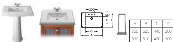
327490000 Basin 750 x 525mm – 1 taphole £352.03 327491000 Basin 630 x 510mm – 1 taphole £283.17 337490000 Pedestal £126.00
