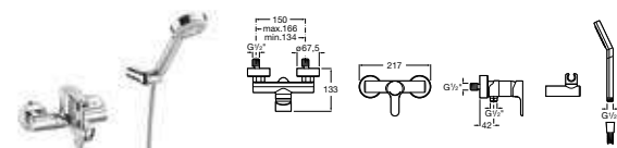
5A0109C00 Wall-mounted bath-shower mixer with kit £102.16
