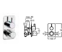
5A2960C00 Built-in thermostatic bath or shower mixer £439.09
