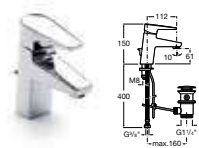
5A3031C00 Basin mixer with pop-up waste £155.81 5A3131C00 Basin mixer £140.23
