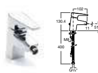
5A6031C00 Bidet mixer with pop-up waste £155.81 5A6131C00 Bidet mixer £140.23
