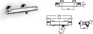
5A1318C00 Wall-mounted thermostatic shower mixer (no kit) £172.22
