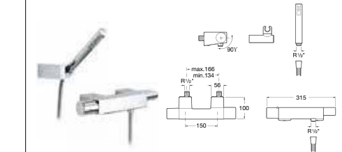
5A1347C00 Wall-mounted thermostatic shower mixer with kit £466.68
