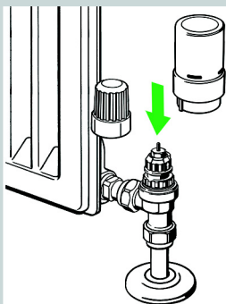
5 Repeat step 3 and 4 until all valves have been set correctly. Sensor may now be fitted or the valve cap temporarily refitted.
