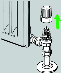
4 Remove cap and turn setting ring according to the drawings - the setting ring is turned by hand only.
