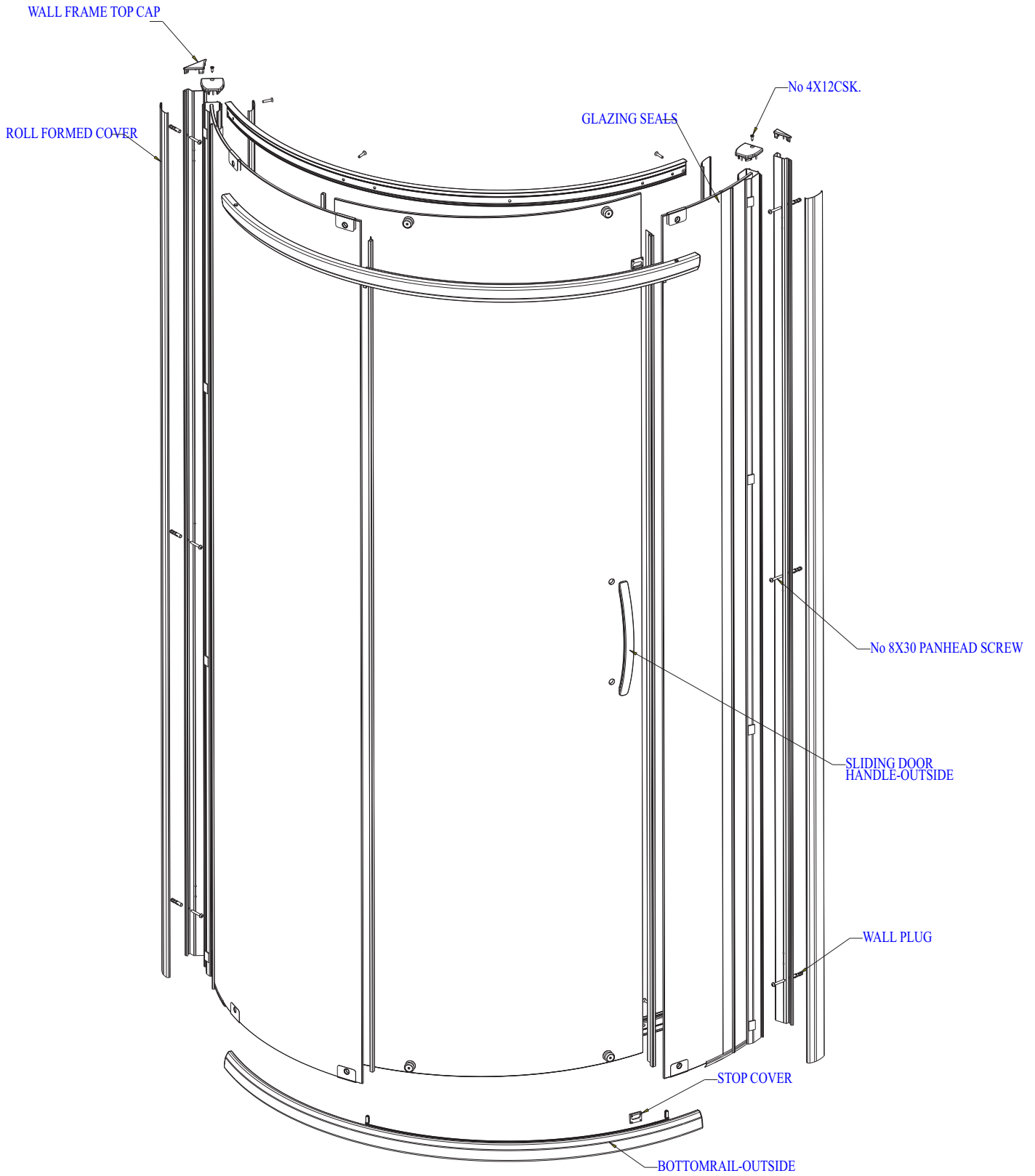
Fig 29 EXPLODED VIEW
