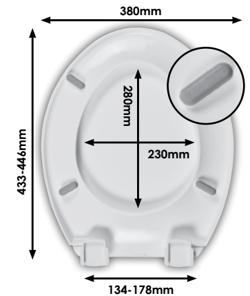
DIAGRAM - SSP11WH Full dimensional details per hinge p37
