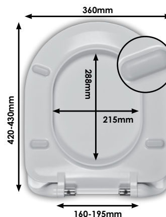
DIAGRAM - 20721280 Full dimensional details per hinge p39
