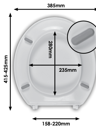
DIAGRAM - 20120361 Full dimensional details per hinge p37
