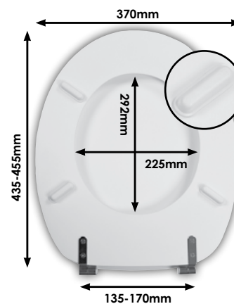
DIAGRAM - 21230004 Full dimensionals details per hinge p39
