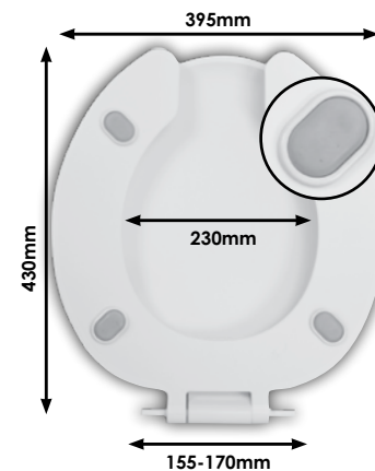
DIAGRAM - SCR12WH Full dimensional details per hinge p39
