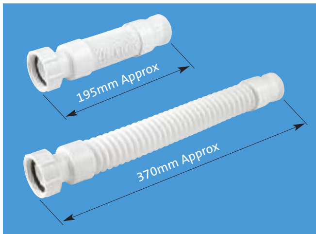
1¼" BSP coupling nut x 1¼" BSP male thread
