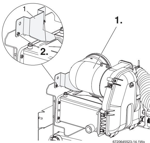
Fig. 20 Securing bracket
