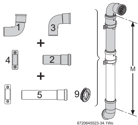
Fig. 33 Optional components in white
