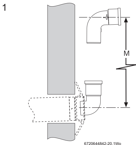
Fig. 39 Plume management length M
