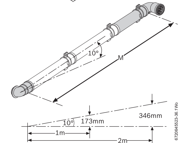
Fig. 35 Plume management with straight extension
