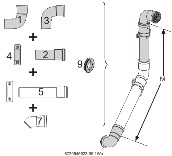
Fig. 34 Plume management with bend
