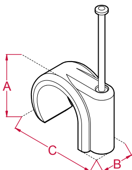
NCW22 22mm Nail Clip A: 27mm B: 15mm C: 36mm Nail Size = 2.0 x 50mm
