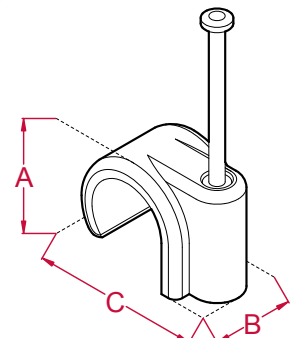
NCW15 15mm Nail Clip A: 20mm B: 15mm C: 27mm Nail Size = 2.0 x 45mm
