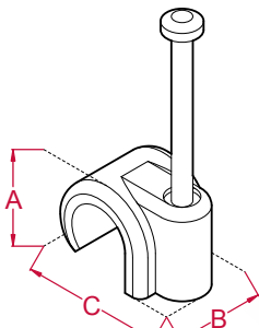
NCW08 7 - 8mm Nail Clip A: 10mm B: 9.5mm C: 14.5mm Nail Size = 2.0 x 25mm
