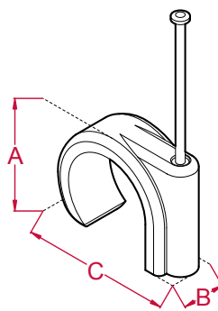
NCW28 28mm Nail Clip A: 33.5mm B: 15mm C: 43mm Nail Size = 2.0 x 55mm
